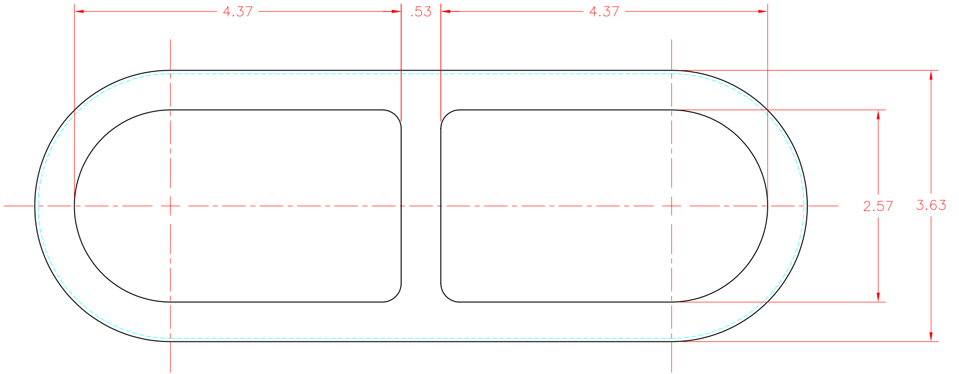
2 PLACE FILTER P/N 080031
